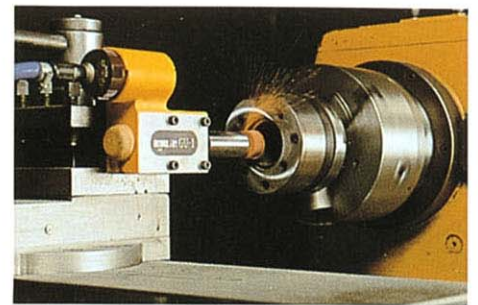
3番軸による内径段付研磨 Internal off-set grinding with No. 3
