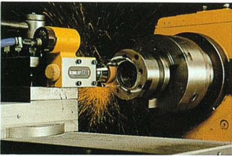
4番軸による端面及び外径同時研磨 End facing and OD grinding, one chucking with No. 4 Spindle
