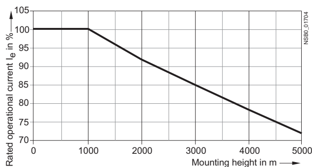
Figure 11-2 Reduction as a function of the installation altitude
